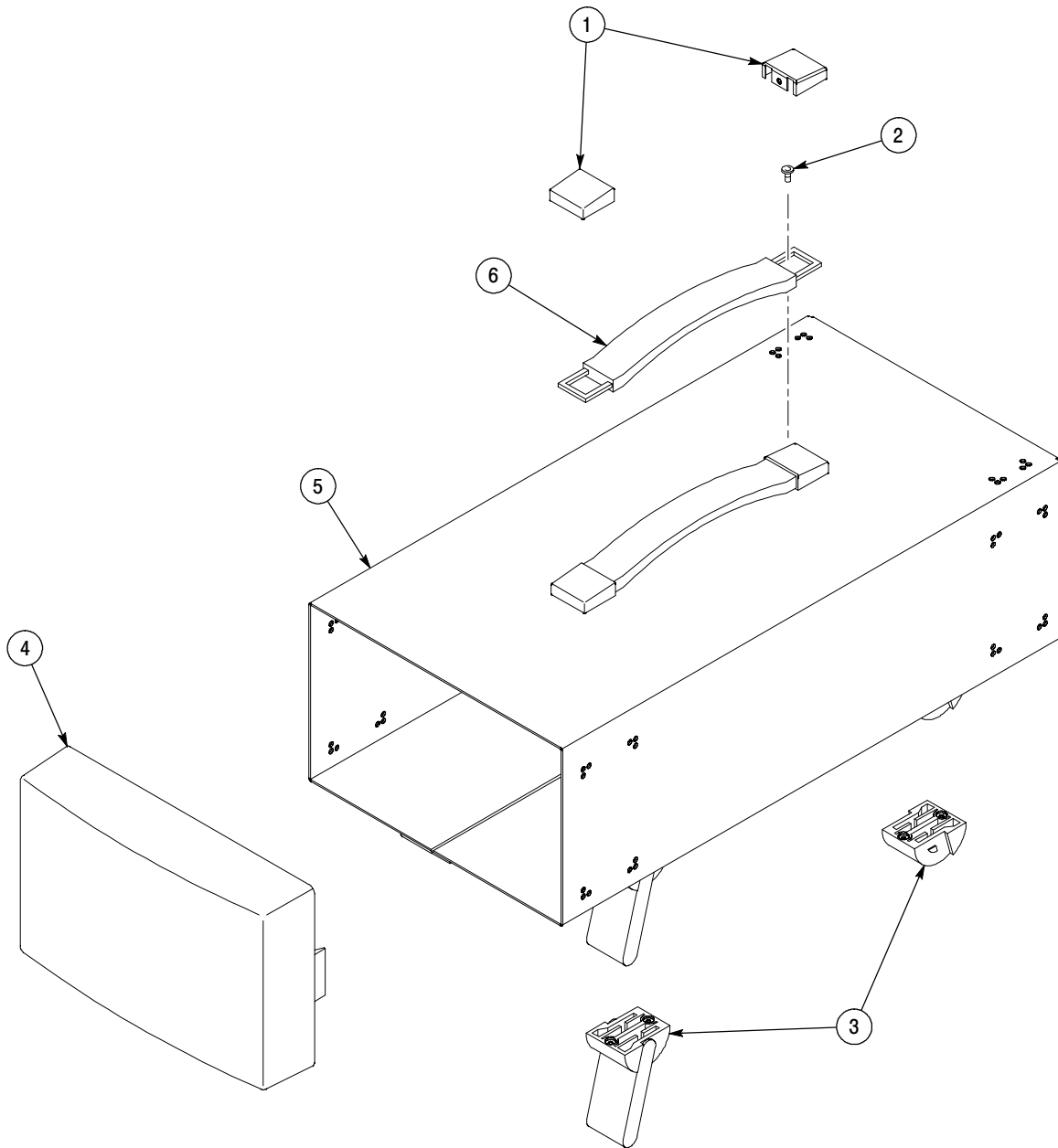
Figure 1: WFM7F02 Exploded view
